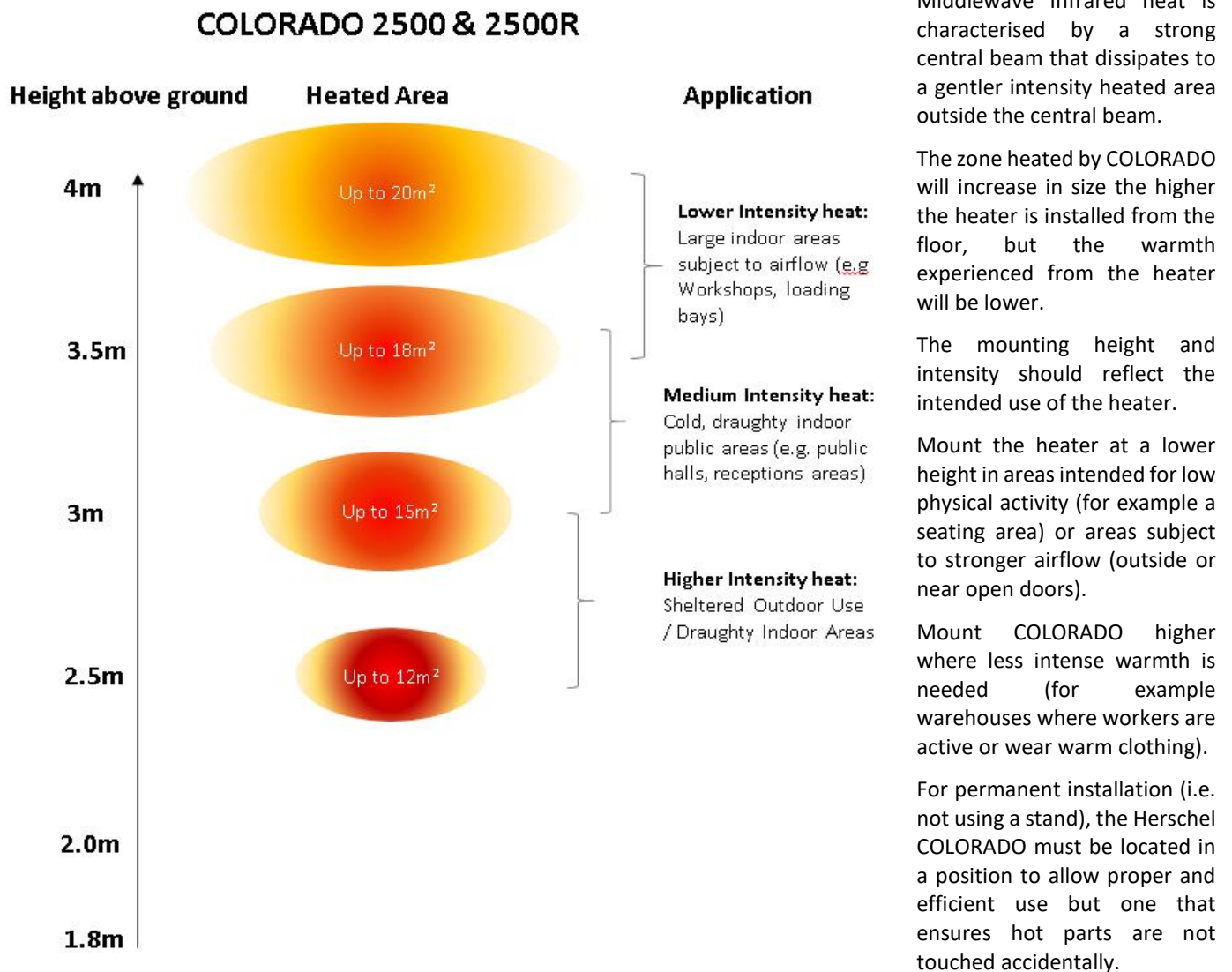
Diagram 1: COLORADO heated area and applications
